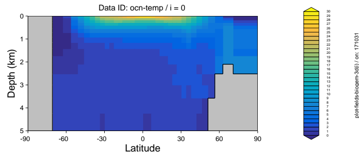
Figure 16.3: Zonal mean global ocean temperature profile.
