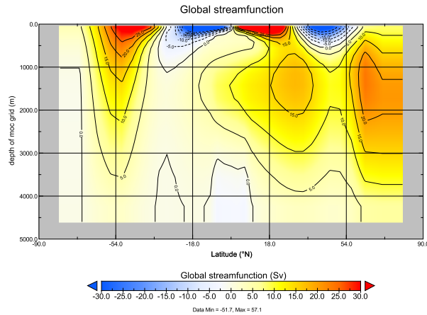
Figure 5.1: Drakework world overturning circulation.
