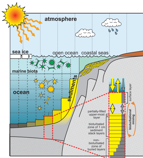
Figure 11.1: Schematic of SEDGEM sediment component.
