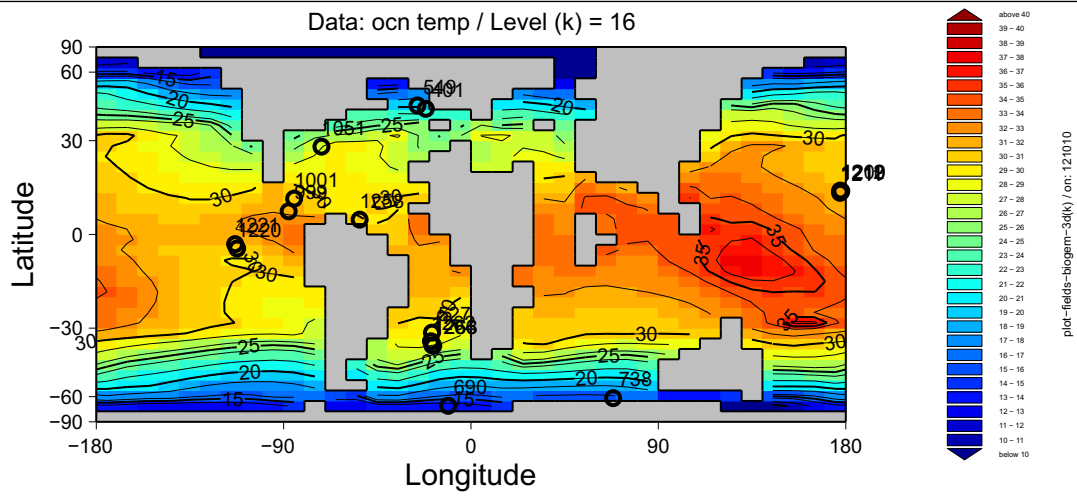
Figure 16.7: Paleocene-Eocene deep-sea sediment drill locations together with a contour-overlain map of surface temperature.
