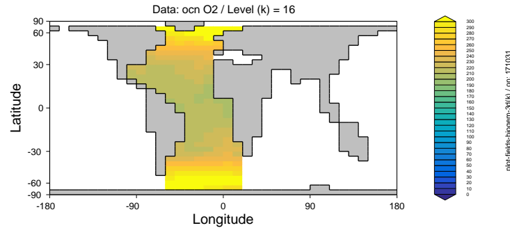
Figure 16.5: Distribution of surface ocean dissolved oxygen in the Atlantic.
