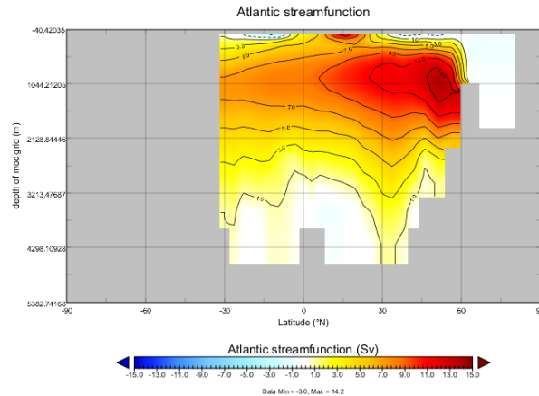
Figure 3.3: Example plot of (normal/default modern) overturning streamfunction (2D netCDF file). (e.g., for Atlantic: netCDF parameter name: phys_ops_ia , long-name: Atlantic streamfunction). Note that autoscaling has been turned off and the min and max plotting limits set manually. By convention, streamfunctions are plotted with their scale symmetrical around zero, giving red and ‘warm’ colors for positive value and clockwise overturning, and blues and ‘cold’ colors for negative values and anti-clockwise overturning. (The plot has been tart-ed up by overlaying solid contours plus contour labels.) It may be necessary in Panoply to re-orient (invert) the vertical grid.
