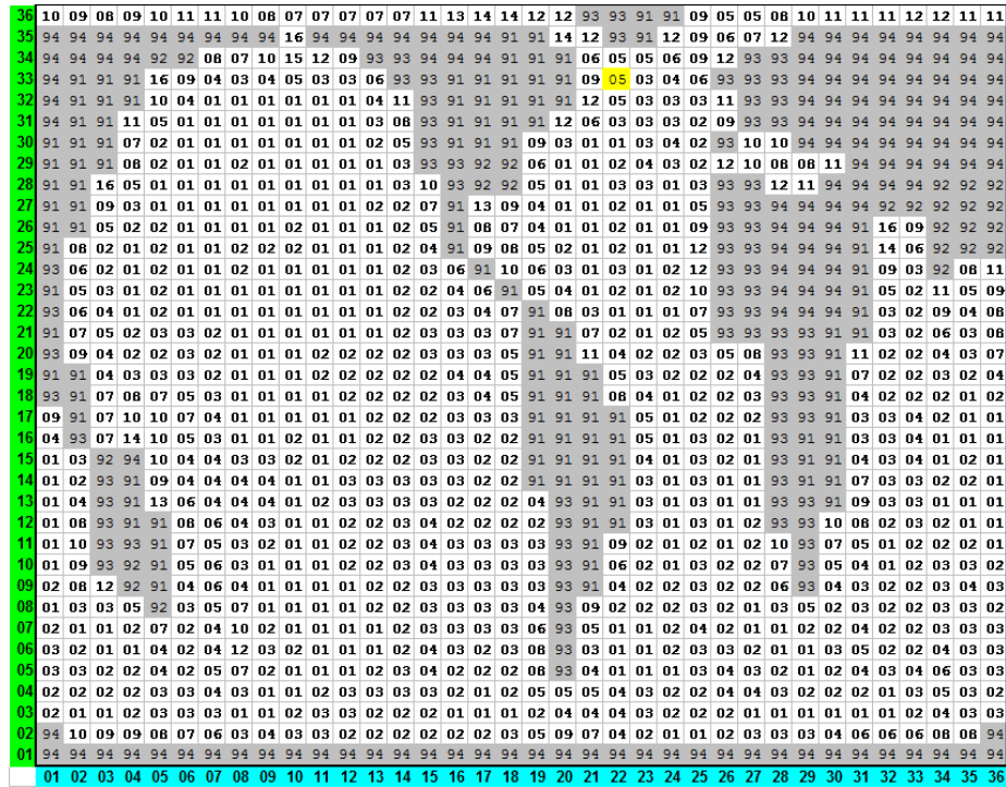
Figure 3.1: The muffin grid for a modern 36 \times 36 ‘worjh2’ configuration. Light blue numbers are the ‘i’ co-ordinates. Green numbers are the ‘j’ co-ordinates. The depth of the ocean at any location is indicated by its ‘k’ value – a number between 1 and 16, with 16 being the surface layer of the ocean, and 1 the maximum possible depth anywhere. Numbers > 90 (91, 92, 93, 94) and shaded grey are land (and specify the direction of run-off). Location (22,33,8) is highlighted in yellow. The longitude of the western edge of this particular modern ocean grid is at 260W, and the increments are 10 degrees.
