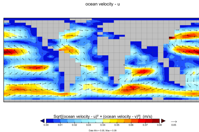
Figure 3.5: Example plot of (normal/default modern) ocean current fields (3D netCDF file). Again scaling has been set manually to create an easy-to-interpret axis scale. On the left is the surface field, and on the right an intermediate depth (illustrating what approximates the Deep Western Boundary current in the model in the Atlantic).
