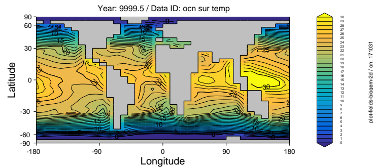
Figure 16.2: Example surface temperature plot, with contours.
