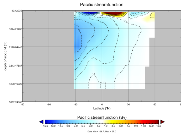
Figure 3.4: Example plot of collapsed AMOC.
