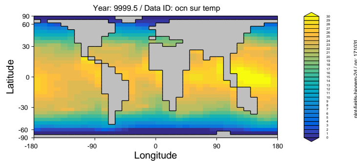
Figure 16.1: Example basic (default) surface temperature plot.
