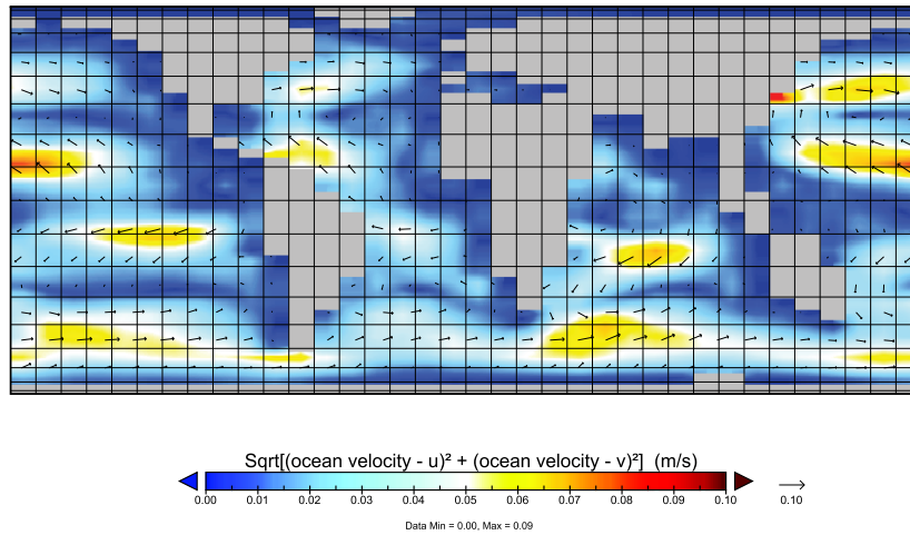
Figure 15.2: Example (modern) ocean surface velocity (current) map.
