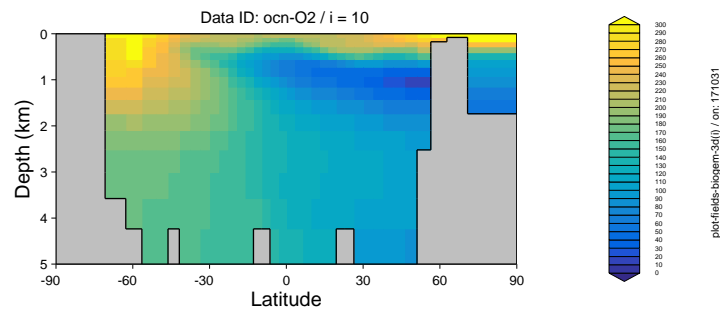
Figure 16.4: Ocean oxygen profile on a Pacific transect.
