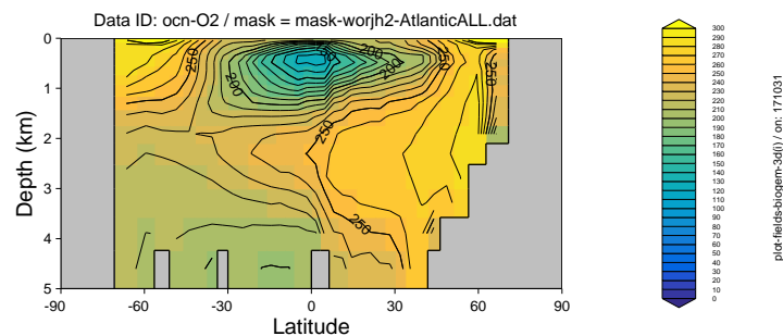
Figure 16.6: Mean zonal ocean oxygen profile in the Atlantic.
