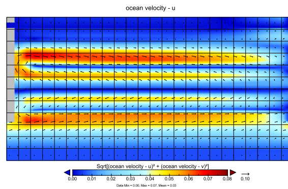
Figure 5.2: Surface current velocity field (arrows) plus speed (color scale).
