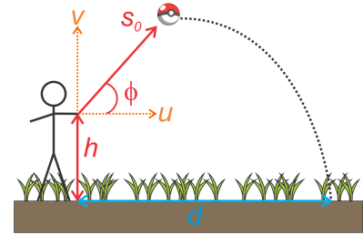
Figure 8.1: Schematic of the thrown-ball system.
