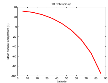
Figure 9.1: Basic 1-D EBM with no latitudinal heat transport and for a single hemisphere only.
