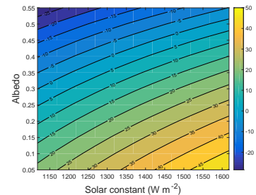
Figure 7.9: Global mean surface temperature ( ^{\circ}C ) as a function of the value of solar constant and surface albedo.
