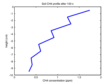
Figure 9.11: Soil profile of CH 4 after 100.0s of simulation with an extremely marginal choice of time-step length.
