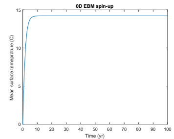
Figure 8.7: 100 yr spin-up of the basic EBM.
