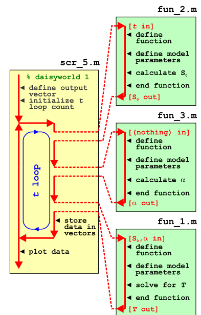
Figure 7.14: Schematic of the evolution of surface temperature over geological time program, and relationship between main program script, the solar constant and EBM functions, and now the 'daisy' albedo function.
