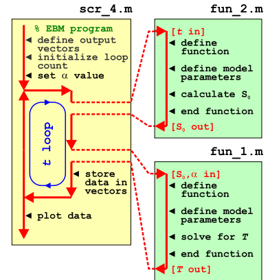
Figure 7.11: Schematic of the evolution of surface temperature over geological time program, and relationship between main program script, and solar constant and EBM functions.
