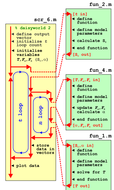
Figure 7.16: Schematic of the evolution of surface temperature over geological time program, and relationship between main program script, the solar constant, EBM, and 'daisy' albedo functions. Note the creation of an inner loop, with EBM, and 'daisy' albedo functions called from within this, while the solar constant remains called from the start of the outer loop as before.
