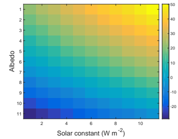
Figure 7.8: Global mean surface temperature ( ^{\circ}C ) as a function of solar constant and surface albedo grid point number.
