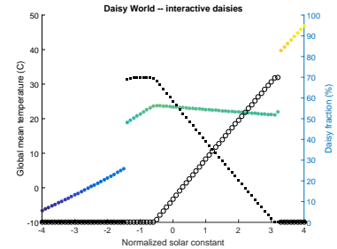
Figure 7.18: Evolution of global surface temperature and the two populations of daisies with time.
