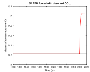
Figure 8.12: Transient EBM response to (fake) changes in atmospheric CO 2 .
