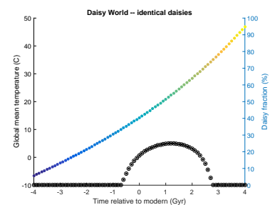
Figure 7.17: Evolution of global surface temperature and the two populations of daisies with time ... but now assuming that the growth of each depends on the global mean surface temperature.
