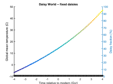
Figure 7.15: Evolution of global surface temperature and the two populations of daisies with time ... but with no change allowed in the daisy populations (d'uh!). The fractional coverage of white daisies is shown by large empty circles, and for black, by small filled black circles. Data points for mean surface temperature are color-coded by temperature (color scale not shown).
