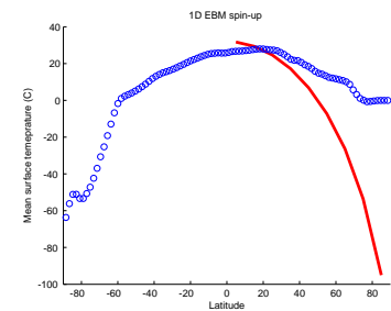
Figure 9.3: As per Figure 9.2 but for July.
