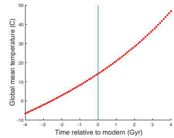
Figure 7.12: Simple EBM projection of the evolution of Earth surface temperature with time. Time at the present-day is highlighted by a vertical line (drawn using the MATLAB line function).
