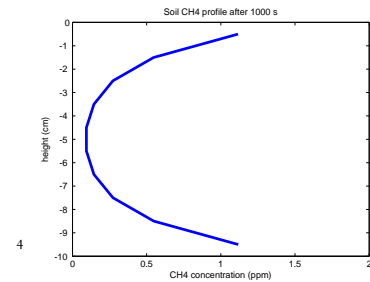
Figure 9.14: Example equilibrium soil profile of CH 4 with production at depth.
