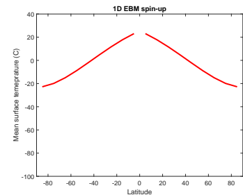
Figure 9.5: 1D EBM with a \times 10 larger value of k .
