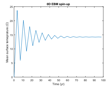
Figure 8.9: 100 yr spin-up of the basic EBM, but with a poor choice of time-step ...
