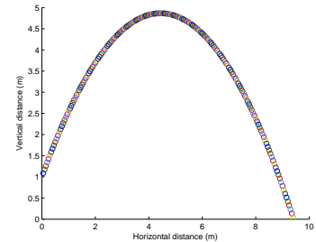
Figure 8.4: Trajectory of a ball!!
