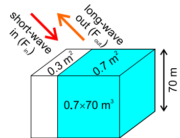
Figure 8.5: Schematic of the dynamic EBM.
