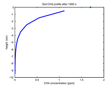
Figure 9.13: Equilibrium soil profile of CH 4 , with CH 4 uptake throughout the soil column with a rate constant of 0.1 per s.
