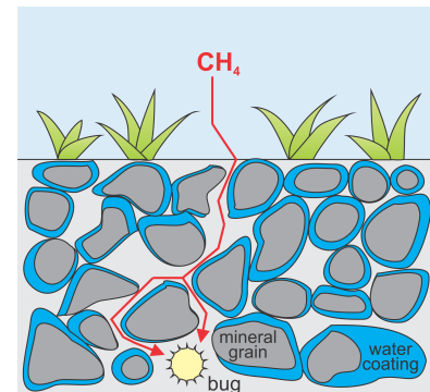
Figure 9.8: Even less idealized and almost realistic, schematic of the soil- \text{CH}_4 system.
