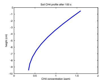
Figure 9.10: Soil profile of \text{CH}_4 after 100.0s of simulation.
