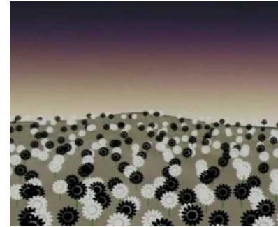
Figure 7.13: Daisy World
