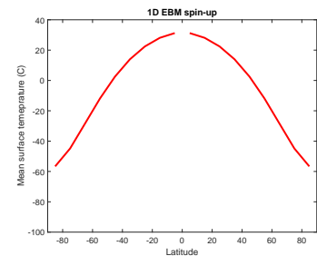
Figure 9.4: 1D EBM with an initial guess as to the value of k .
