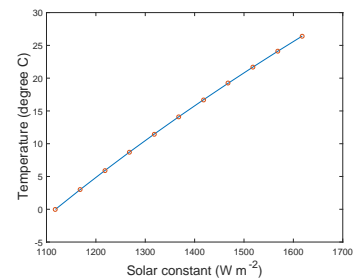
Figure 7.5: Sensitivity of global mean surface temperature vs. solar constant (mean surface albedo held constant at an albedo value of 0.3).
