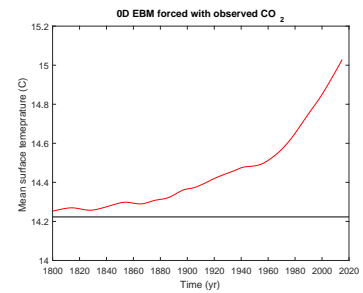
Figure 8.11: Transient EBM response to observed changes in atmospheric CO 2 . For reference, the pre-industrial equilibrium global temperature is shown as a horizontal black line.
