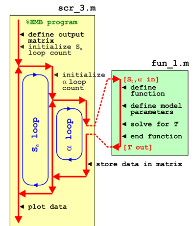
Figure 7.7: Schematic structure of the model configured to carry out a double (in terms of solar constant AND now albedo) parameter sensitivity study.
