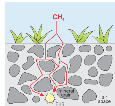
Figure 9.7: Slightly less idealized schematic of the soil- \text{CH}_4 system.
