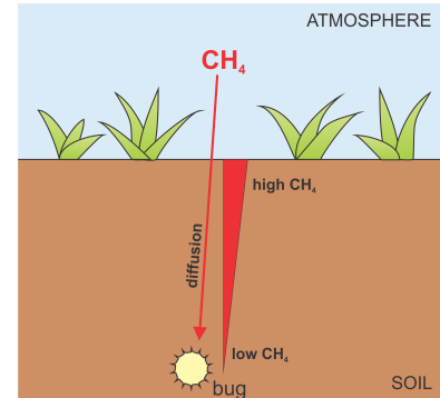
Figure 9.6: Idealized schematic of the soil- \text{CH}_4 system.
